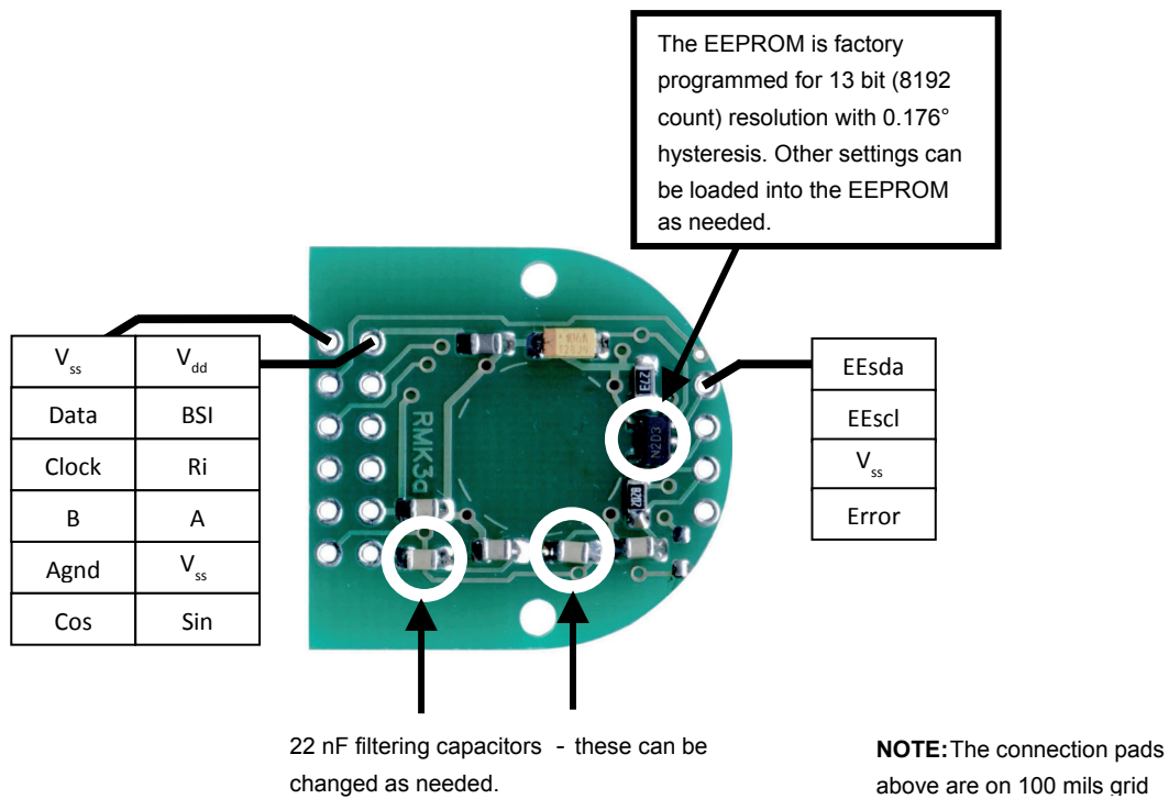
Fig. 35: RMK3B pin assignment
