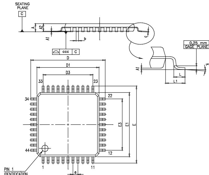
Fig. 34: LQFP44 package dimensions
