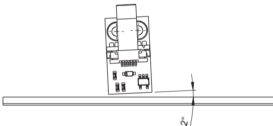
Yaw
