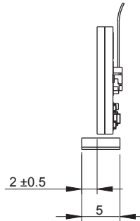
Lateral offset
