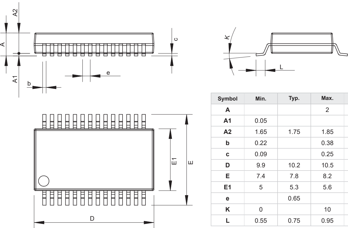
Fig. 32: Dimensional drawing
