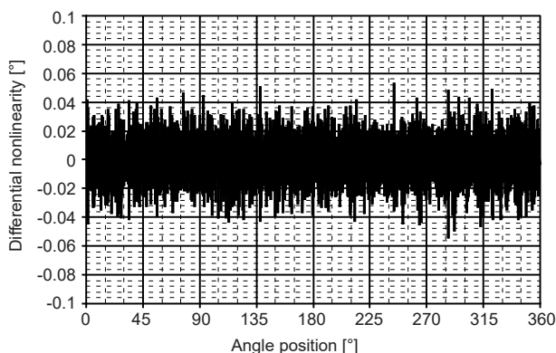
Fig. 24: Typical differential nonlinearity
