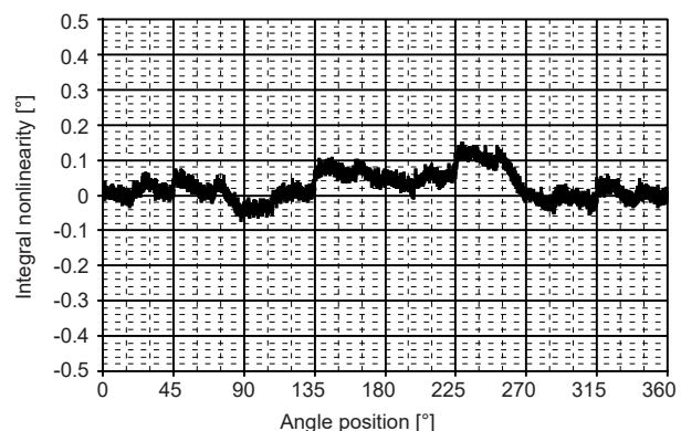
Fig. 25: Typical integral nonlinearity at optimal parameters
