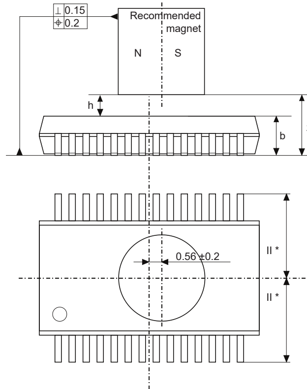
Fig. 30: Mounting instructions
