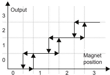
Fig. 7: Hysteresis
