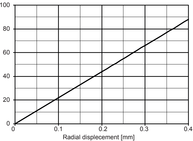
Fig. 19: Error signal amplitude
