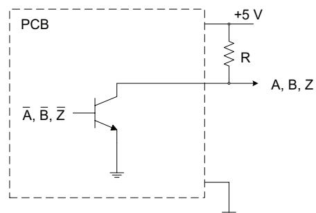
Recommended signal termination
