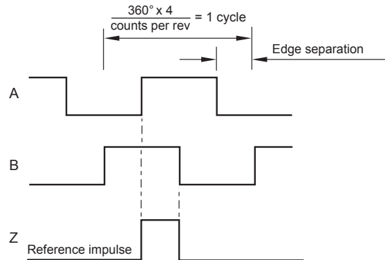
Timing diagram
