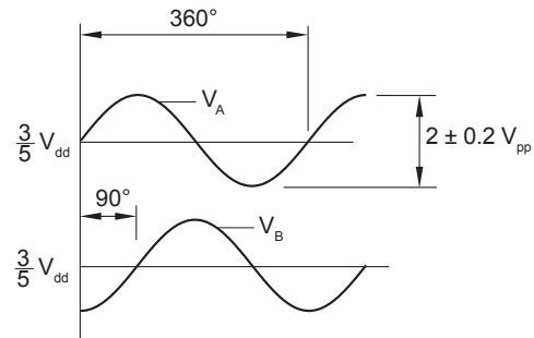
Timing diagram
