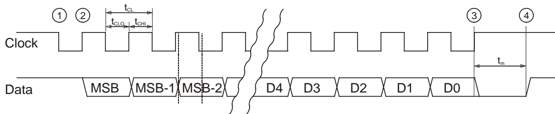
Fig. 7: SSI timing diagram
