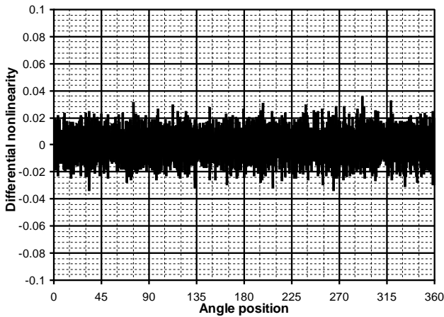
Fig. 15: Typical differential nonlinearity
