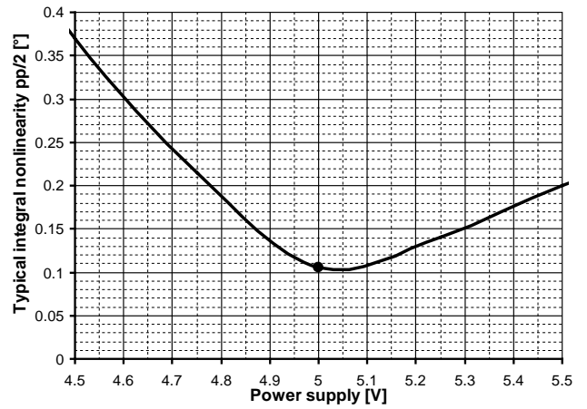
Fig. 29: Accuracy Vs Power supply
