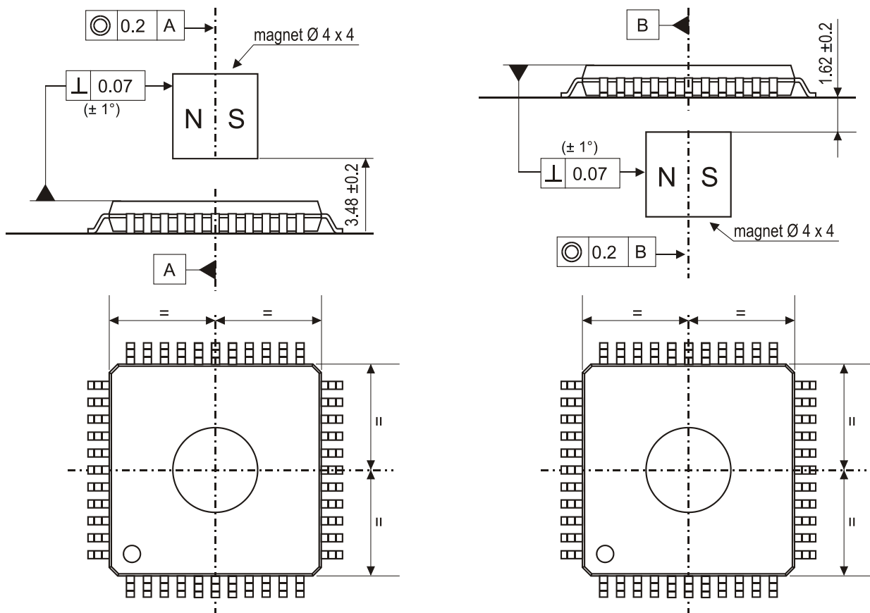
Fig. 24: Mounting instructions
