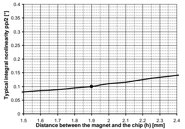
Fig. 31: Accuracy Vs Distance
