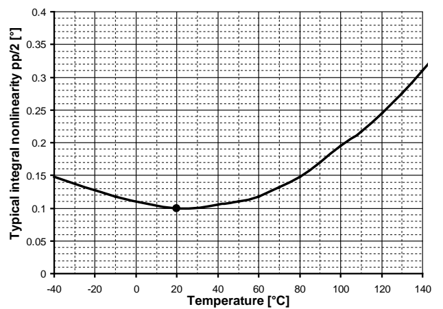
Fig. 33: Accuracy Vs Temperature
