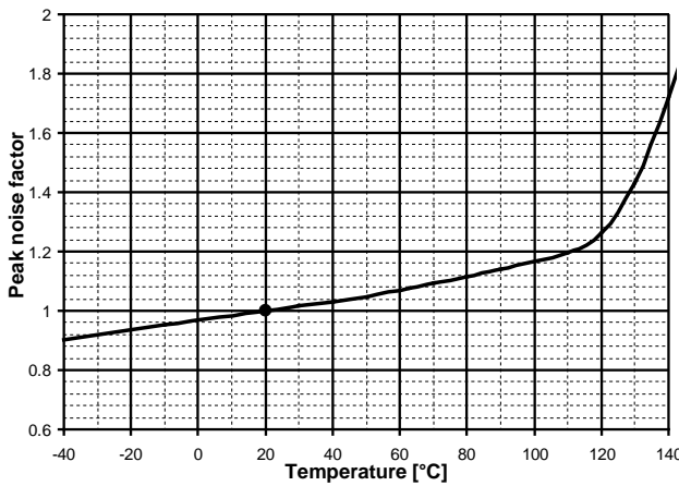
Fig. 13: Peak noise factor Vs Temperature *
