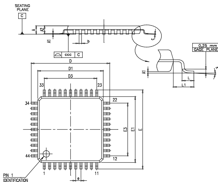
Fig. 35: LQFP44 package dimensions
