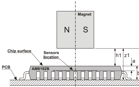
Fig. 22: Magnet placed above the AM8192B
