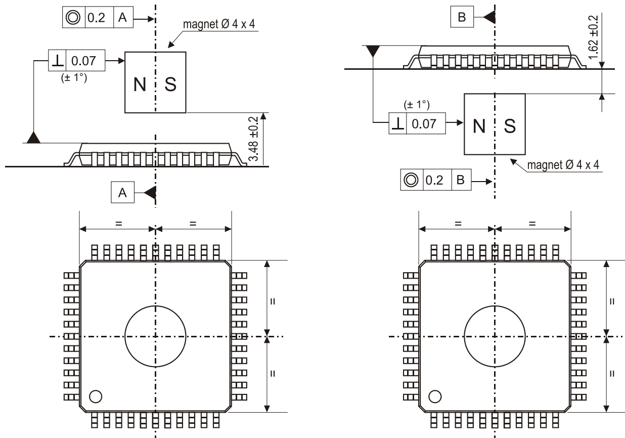
Fig. 24: Mounting instructions
