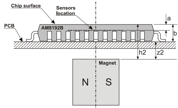
Fig. 23: Magnet placed below AM8192B
