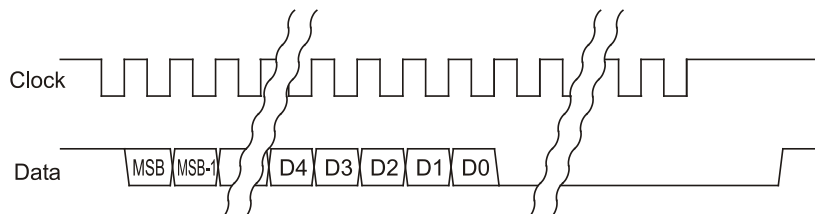
Fig. 9: SSI no ring register mode
