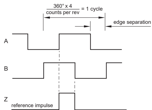
Timing diagram
