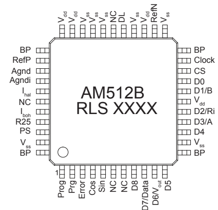
Fig. 1: Pin description
