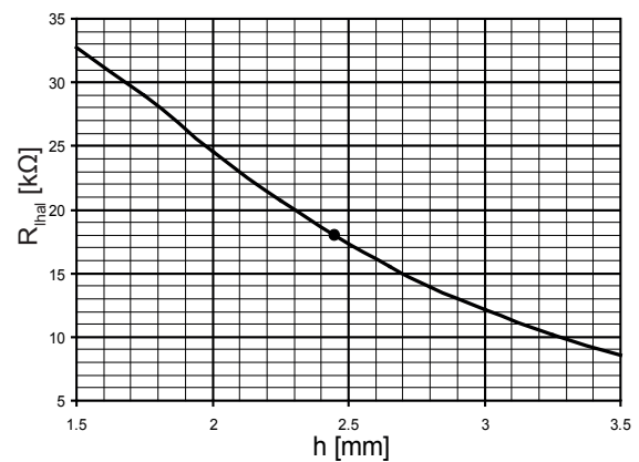
Fig. 34: R_{Ihal} to maintain signal amplitude at different h
