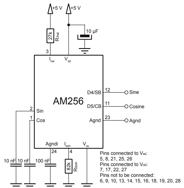
Fig. 23: Buffered analogue output (for AM256S only)
