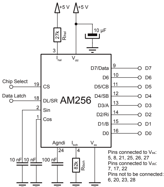
Fig. 20: Parallel output
