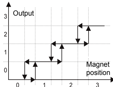
Fig. 7: Hysteresis
