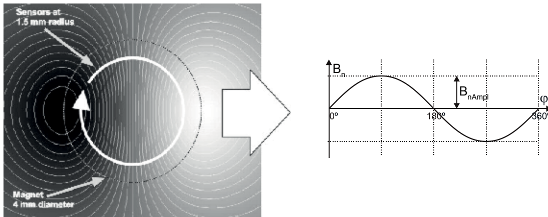
Fig 13: Distribution of B_n and its modulation if the magnet is rotated through 360°
