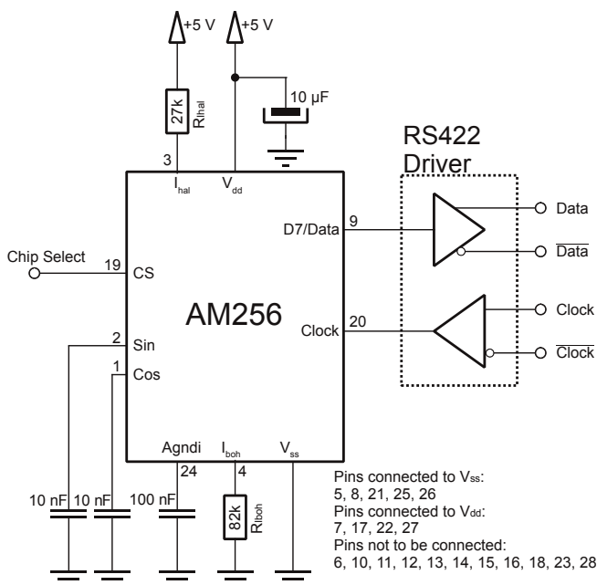
Fig. 22: SSI output
