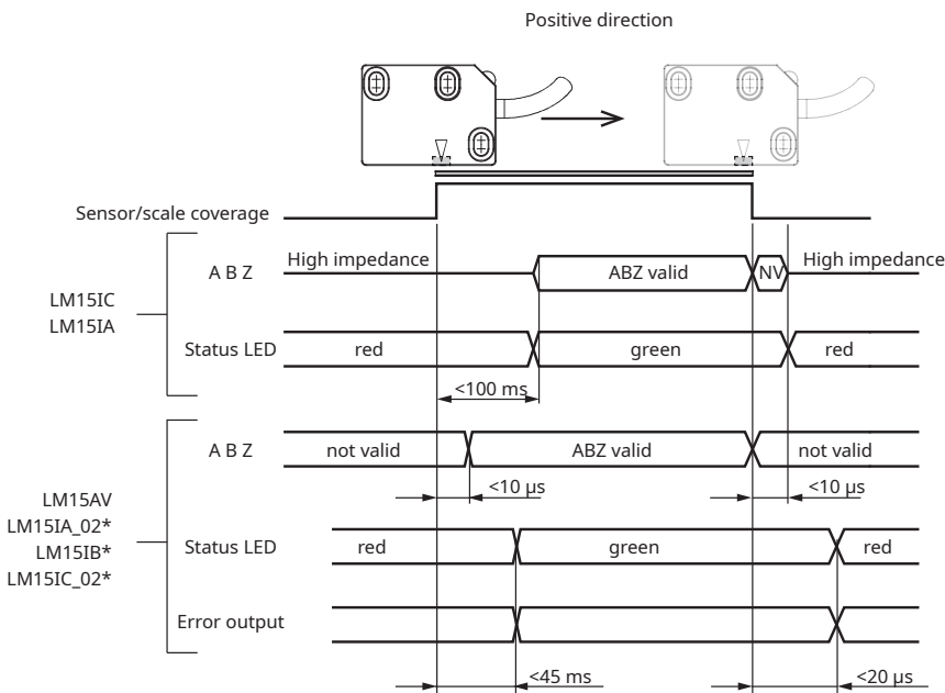
Diagram 2: Transition time
